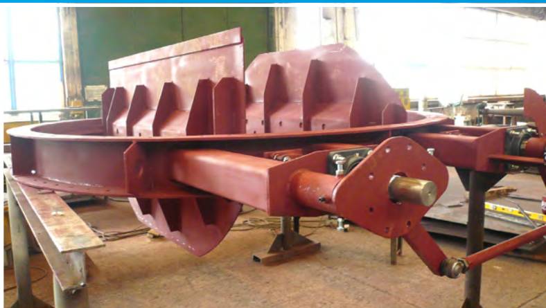
KW Bexbach Mill safety damper type, 4 pcs. Material 16Mo3 Dimension lw. 1520 x 1520 2010
